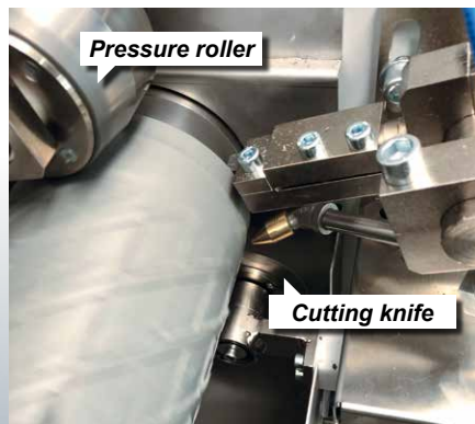
Electrical monitoring of the pressure roller and cutting knife
